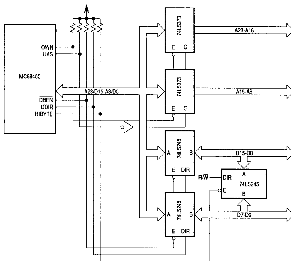
Figure 10. Demultiplex Logic
