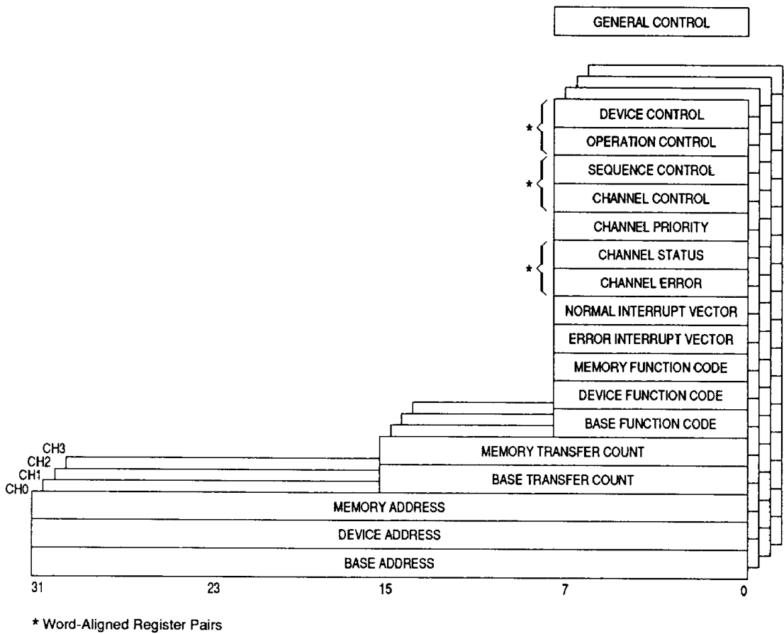
Figure 8. Programmer's Model
