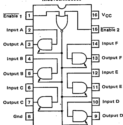
MC8T95/MC6885
