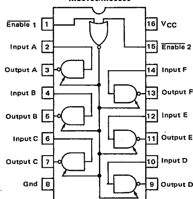
MC8T96/MC6886
