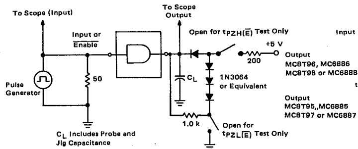
FIGURE 1 - TEST CIRCUIT FOR SWITCHING CHARACTERISTICS
