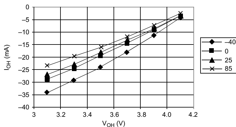
Figure 23-3. Typical High-Side Driver Characteristics – Port PTC1–PTC0 ( V_{DD} = 4.5 \text{ Vdc} )
