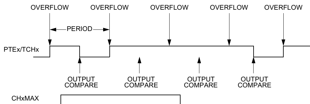
Figure 22-13. CHxMAX Latency
