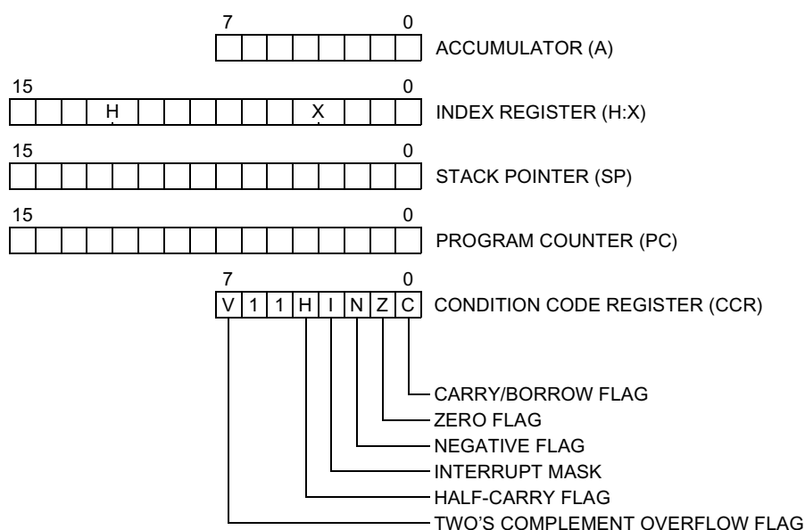
Figure 10-1. CPU registers
