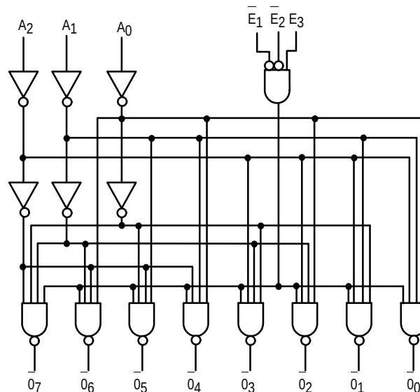
LOGIC DIAGRAM
