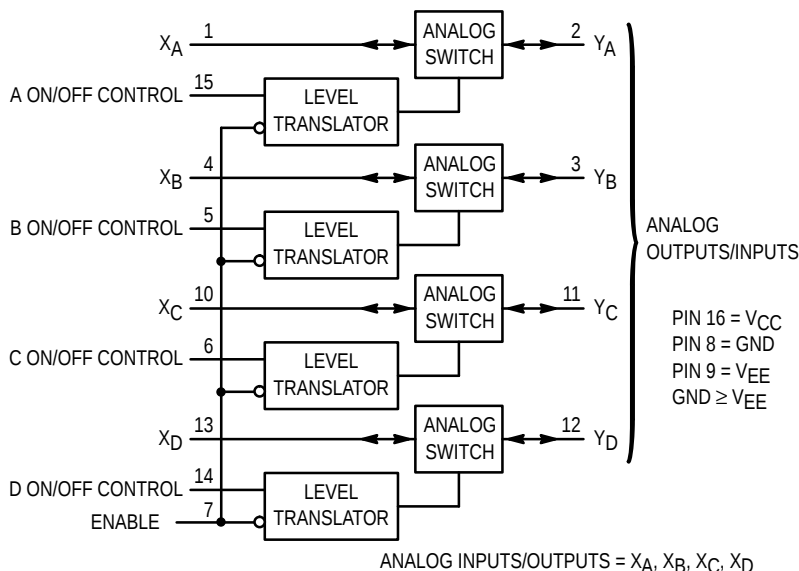
LOGIC DIAGRAM
