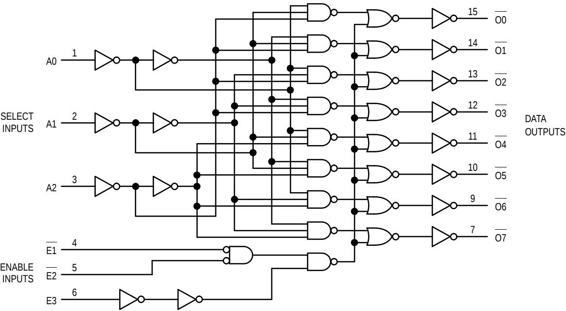
Figure 2. Logic Diagram
