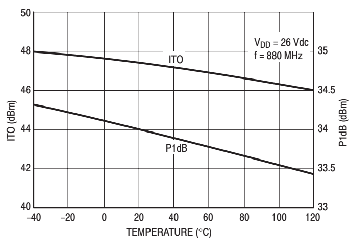
Figure 4. ITO, P1\text{dB} versus Temperature
