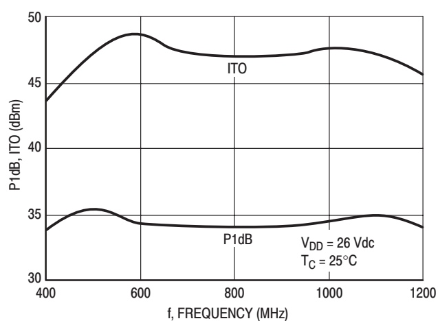
Figure 2. P1\text{dB} , ITO versus Frequency
