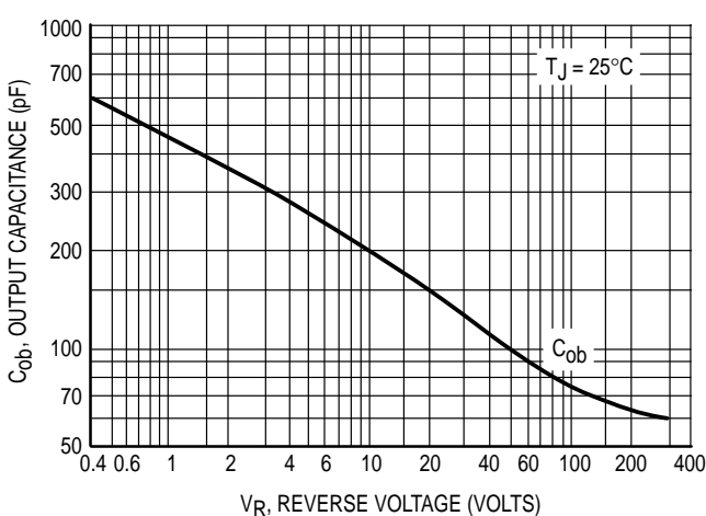
Figure 6. Output Capacitance
