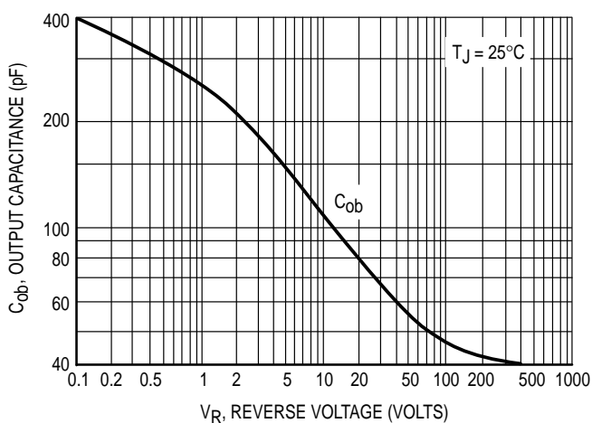
Figure 6. Output Capacitance
