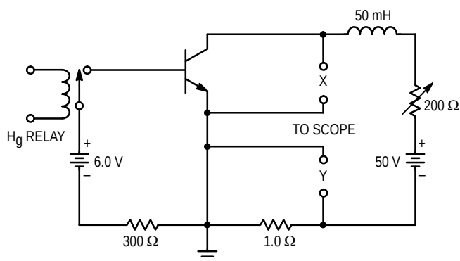
Figure 5. Sustaining Voltage Test Circuit
