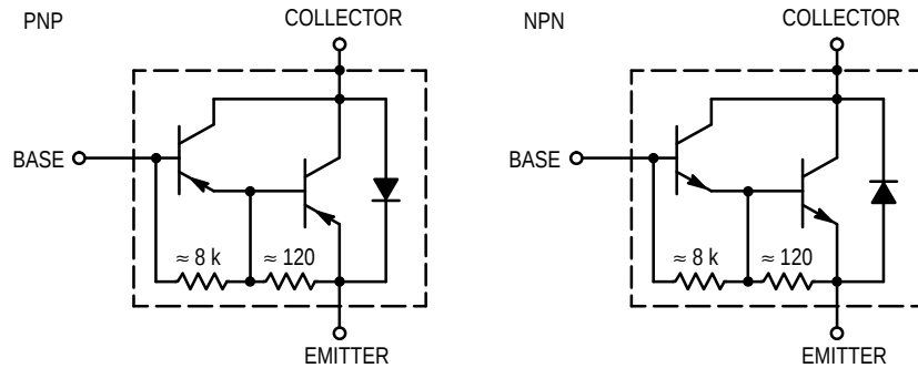
Figure 12. Darlington Schematic
