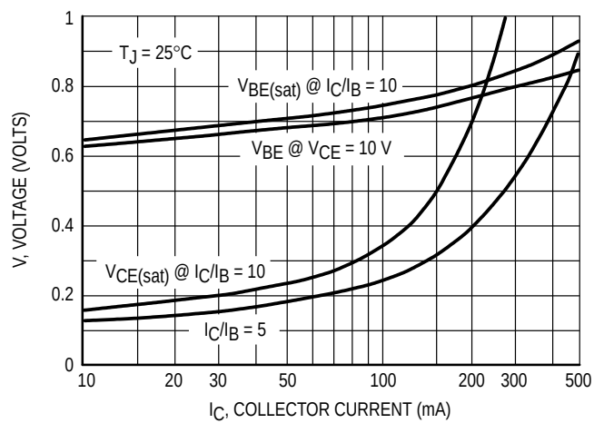
Figure 2. "On" Voltages
