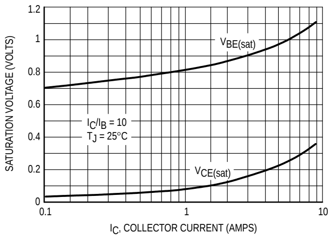
Figure 8. MJD44H11 On-Voltages
