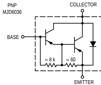
Figure 12. Darlington Schematic
