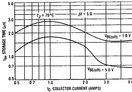
FIGURE 9 — STORAGE TIME
