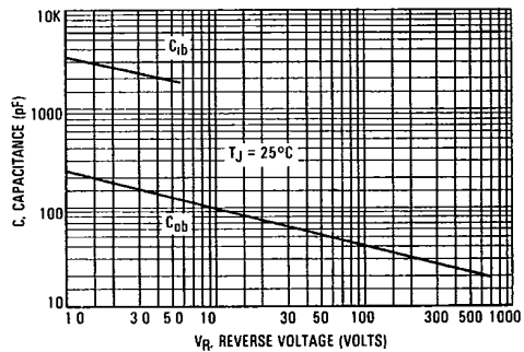
FIGURE 6 — CAPACITANCE
