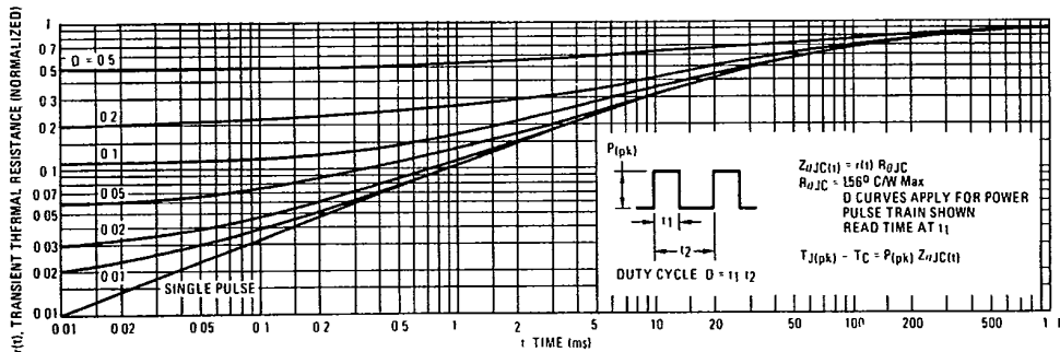
FIGURE 11 — THERMAL RESPONSE
