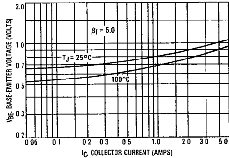
FIGURE 4 — BASE-EMITTER VOLTAGE
