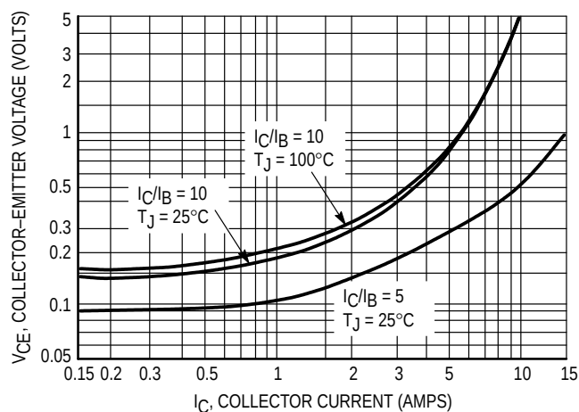
Figure 2. Collector-Emitter Saturation Region
