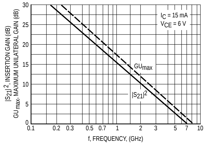
Figure 6. MRF9411LT1
