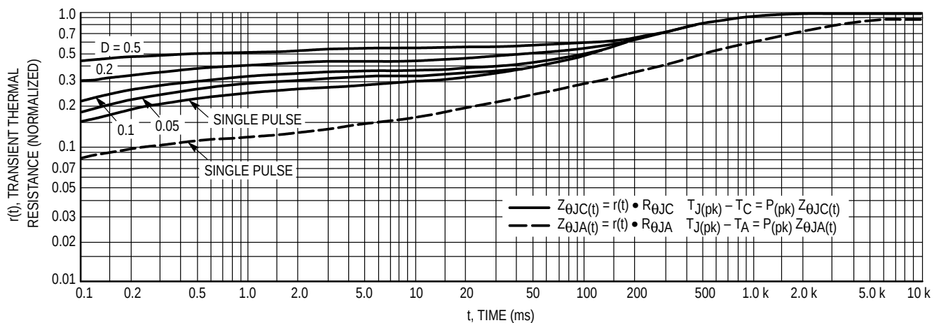
Figure 9. Thermal Response
