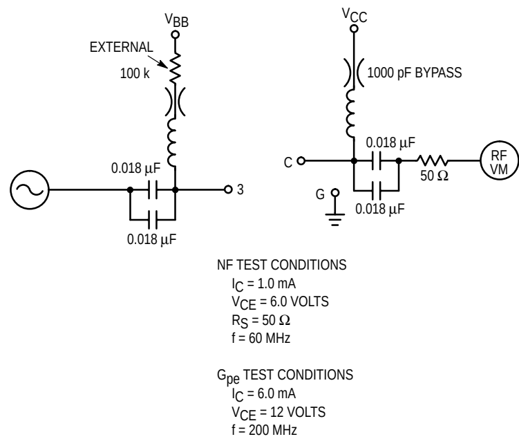
Figure 1. NF, G pe Measurement Circuit 20–200
