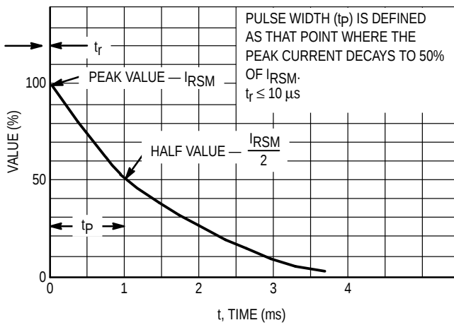
Figure 7. Pulse Waveform
