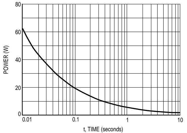
Figure 17. Single Pulse Power
