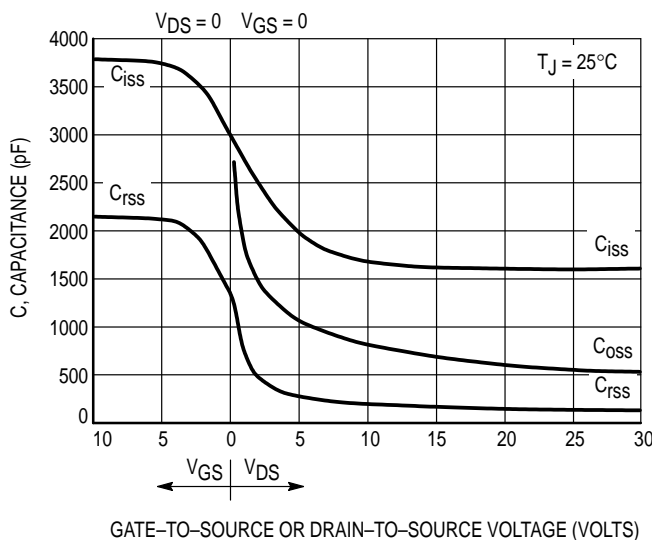
Figure 7. Capacitance Variation
