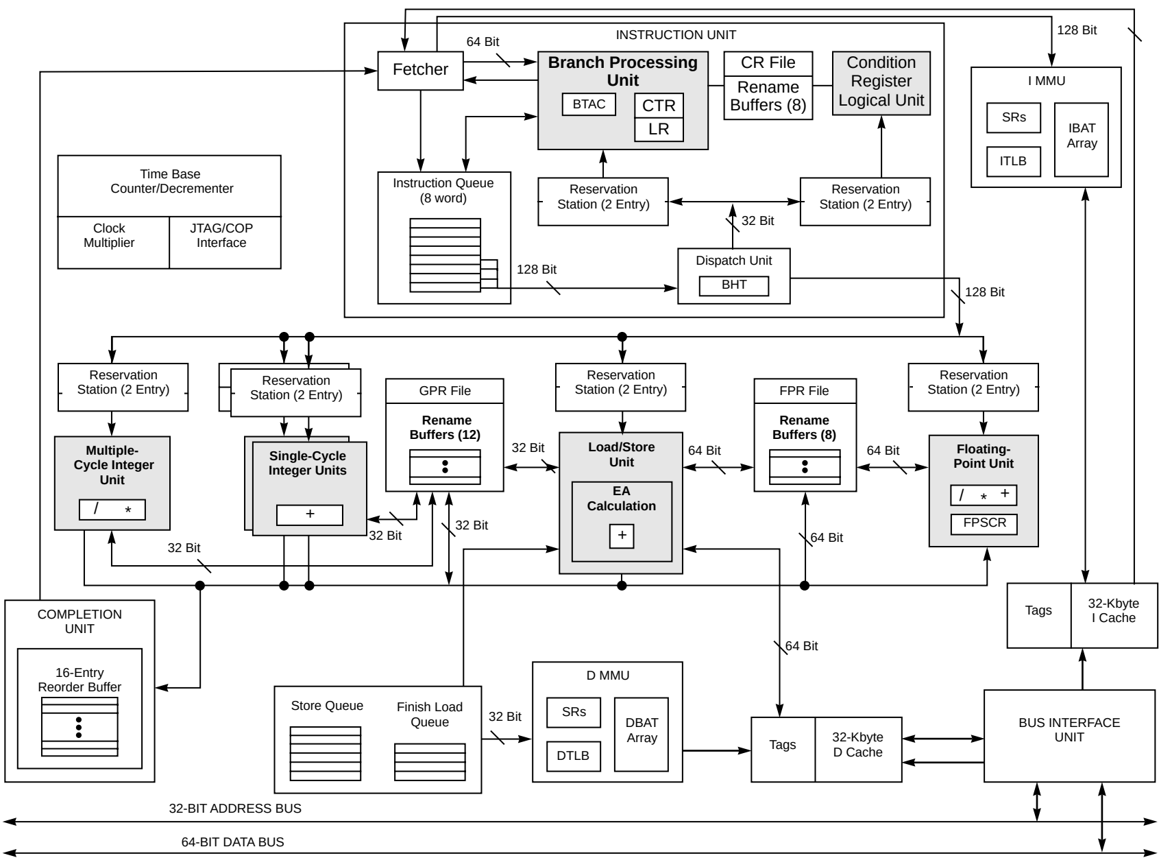
Figure 1. Block Diagram
