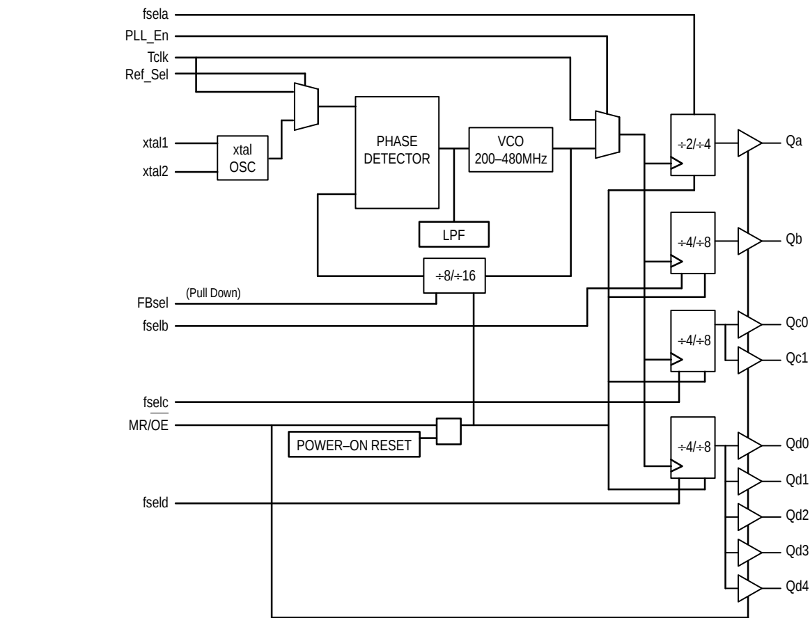
MPC950 LOGIC DIAGRAM
