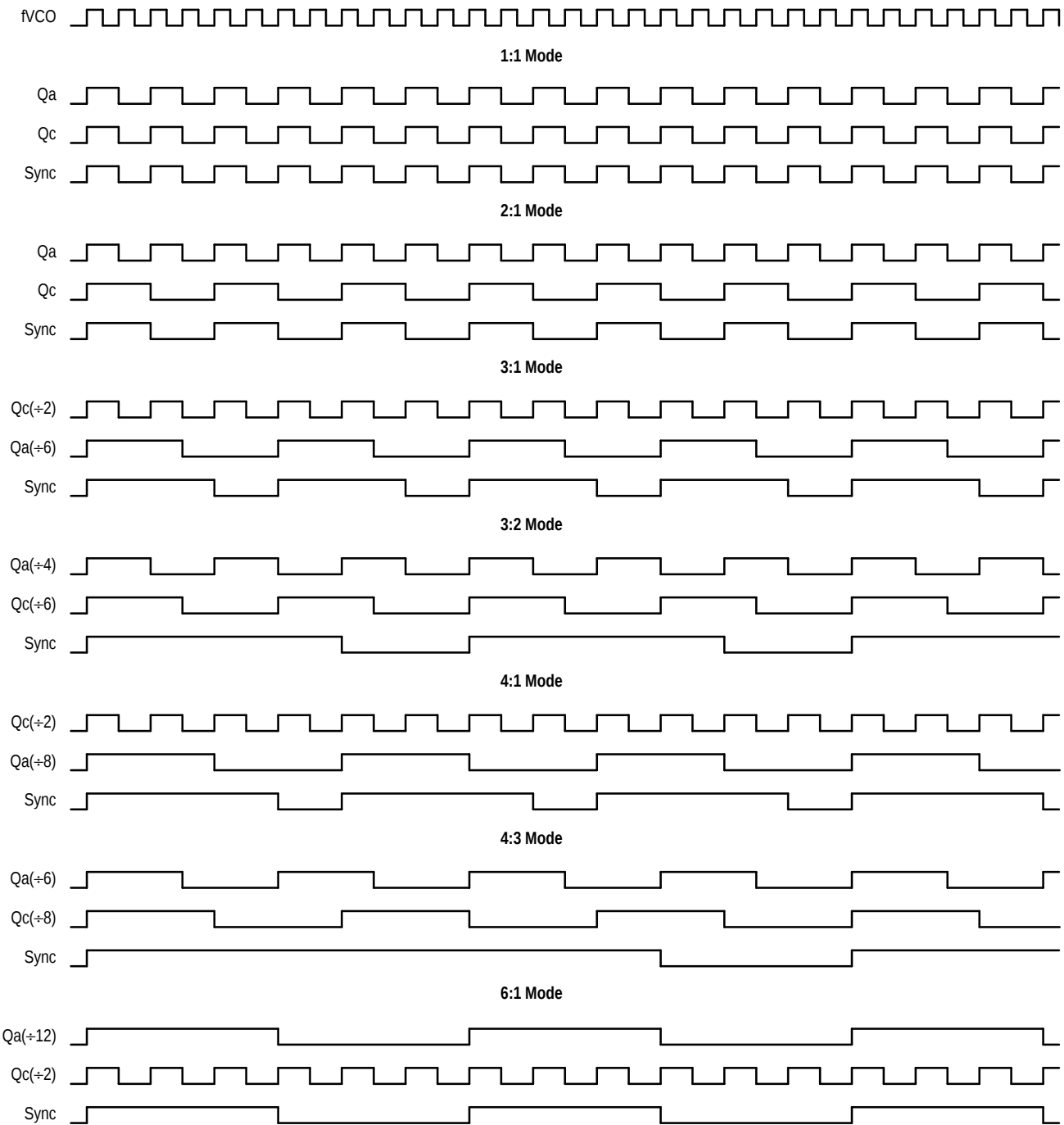
Figure 3. Timing Diagrams
