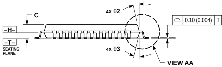
VIEW AA
