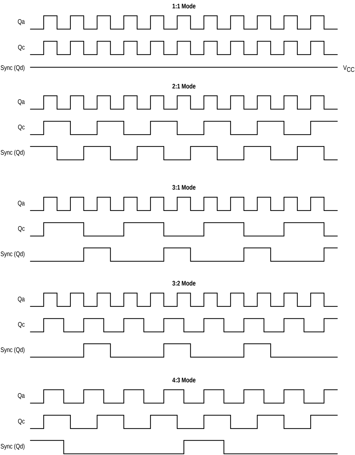
Figure 3. Timing Diagrams
