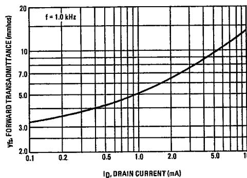
FIGURE 2 - FORWARD TRANSMITTANCE
