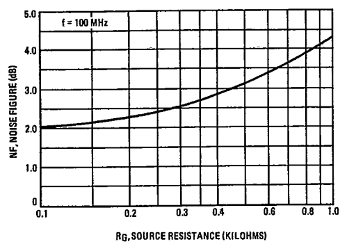
FIGURE 1 - NOISE FIGURE
