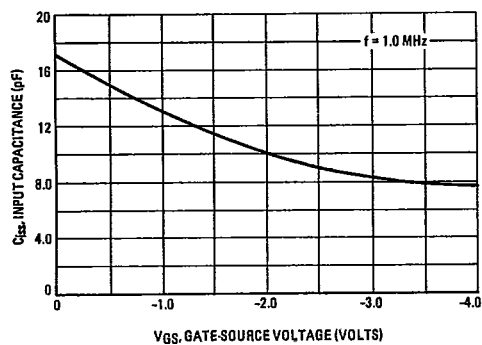
FIGURE 3 - INPUT CAPACITANCE
