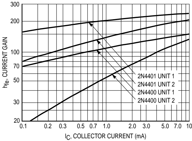
Figure 11. Current Gain
