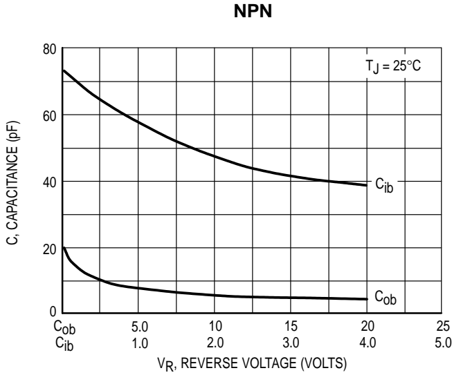
Figure 8. Capacitance
