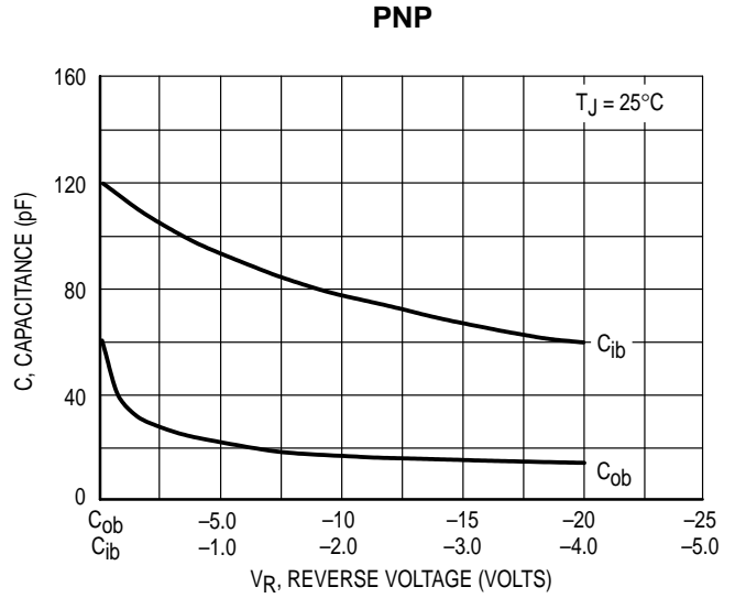
Figure 9. Capacitance
