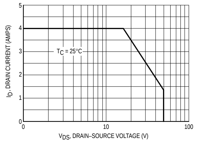
Figure 19. Maximum Rated Forward Biased Safe Operating Area
