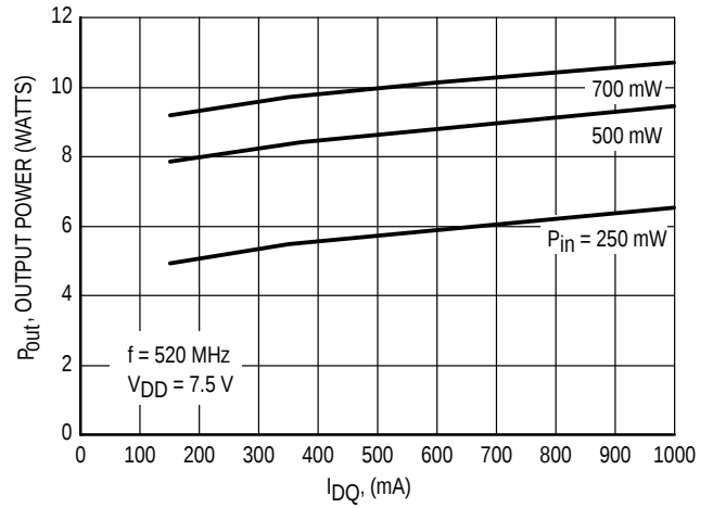
Figure 13. P_{out} versus I_{DQ}
