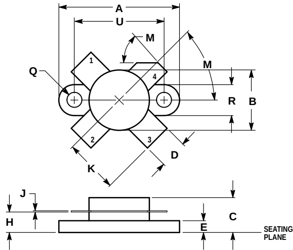
CASE 211-11 ISSUE N
