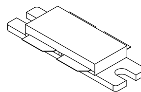
CASE 375B-02, STYLE 2
