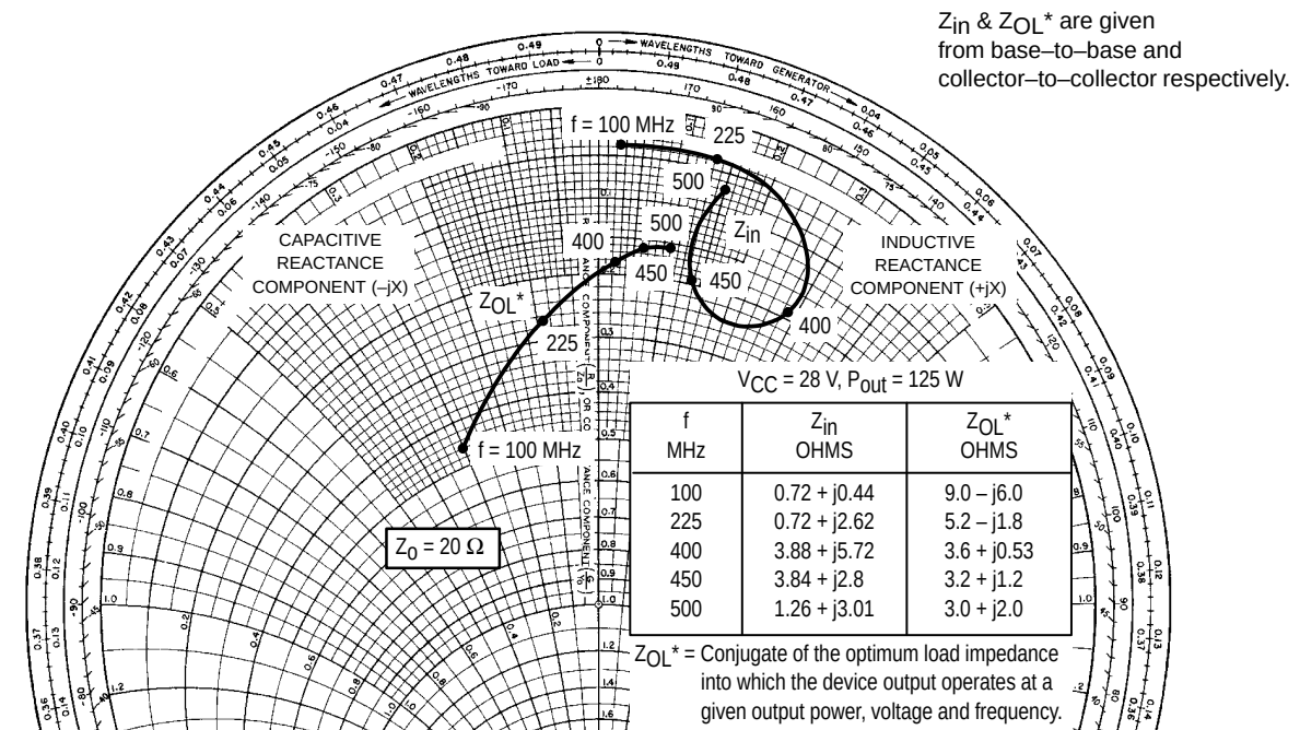
Figure 6. Series Equivalent Input/Output Impedance
