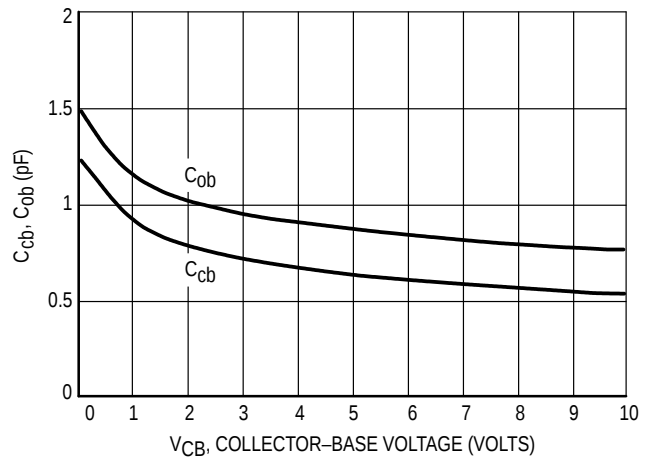
Figure 3. Output Capacitance versus Collector-Base Voltage
