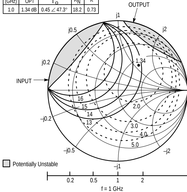
Figure 21. MRF949T1 Series Constant Gain and Noise Figure Contours
