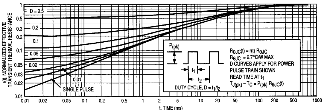
Figure 10. Thermal Response
