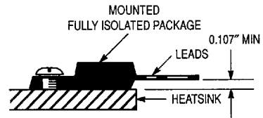
Figure 21. Screw Mounting Position for Isolation Test Number 3
