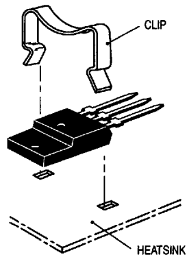
22b. Clip-Mounted
