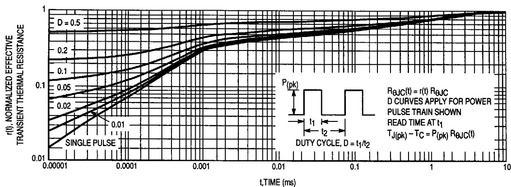
Figure 13. Thermal Response
