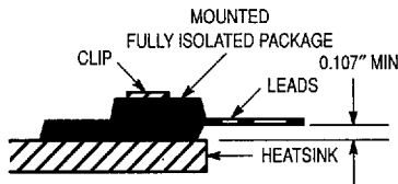
Figure 20. Clip Mounting Position for Isolation Test Number 2
