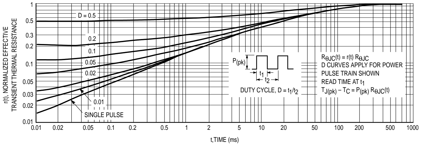
Figure 13. Thermal Response
