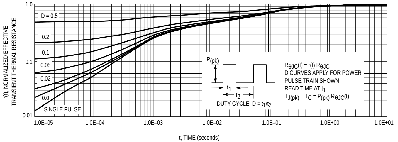
Figure 13. Thermal Response
