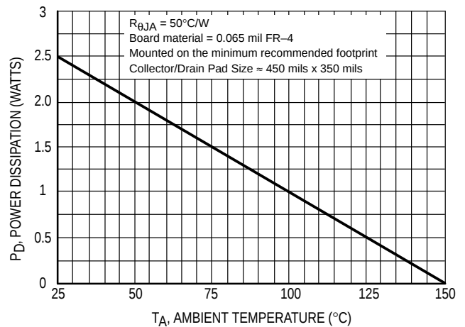
Figure 15. D²PAK Power Derating Curve
