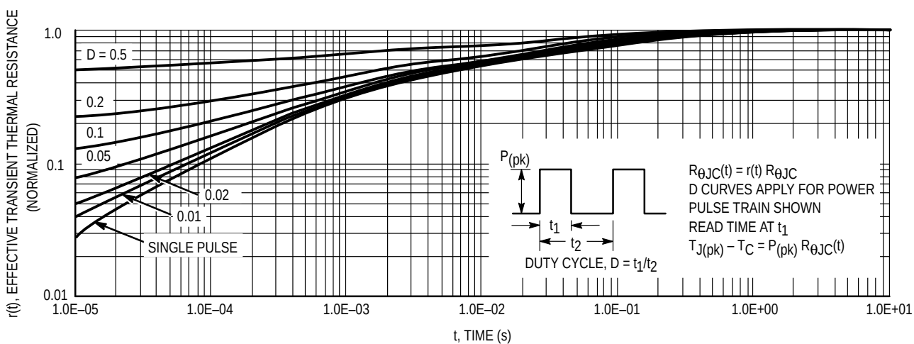
Figure 14. Thermal Response
