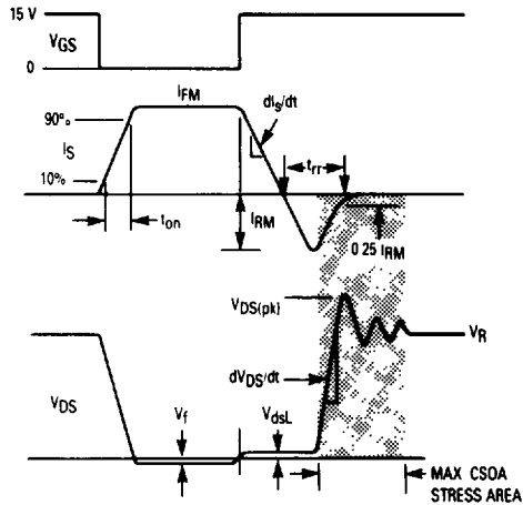
Figure 12. Commutating Safe Operating Area Test Circuit
