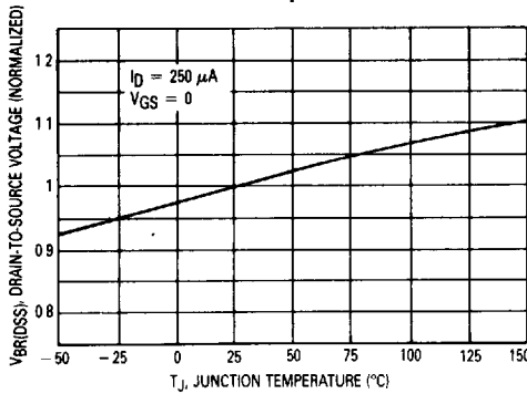
Figure 7. Breakdown Voltage Variation With Temperature
