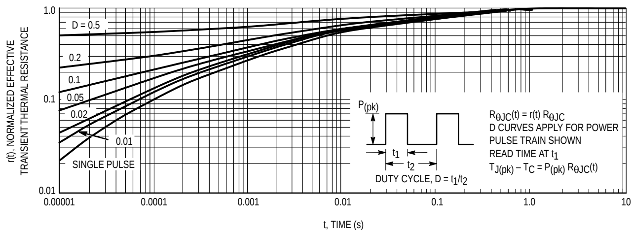
Figure 13. Thermal Response
