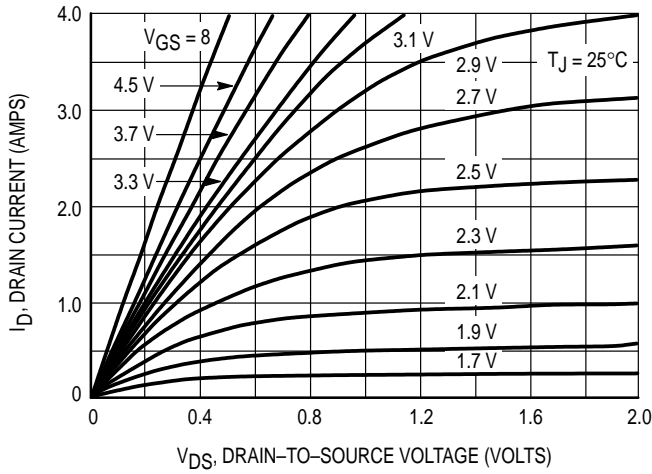
Figure 3. On-Region Characteristics
