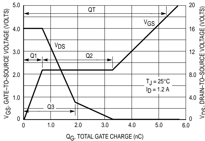
Figure 10. Gate-to-Source and Drain-to-Source Voltage versus Total Charge
