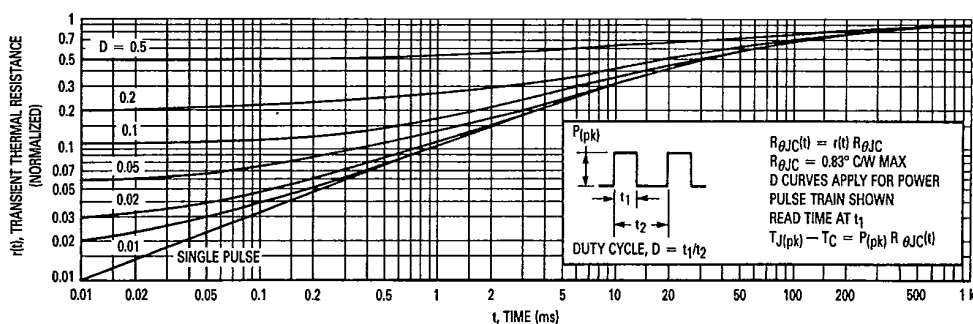
Figure 10. Thermal Response
