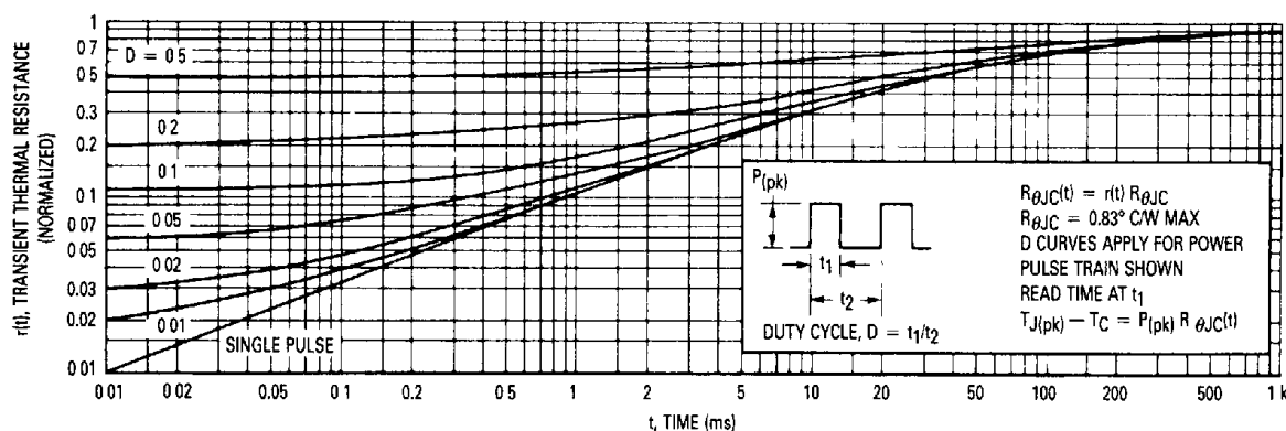
Figure 10. Thermal Response
