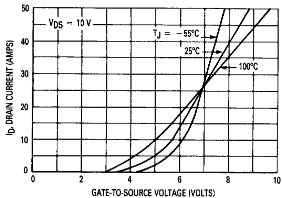
Figure 3. Transfer Characteristics
