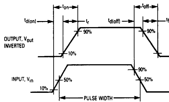
Figure 14. Switching Waveforms
