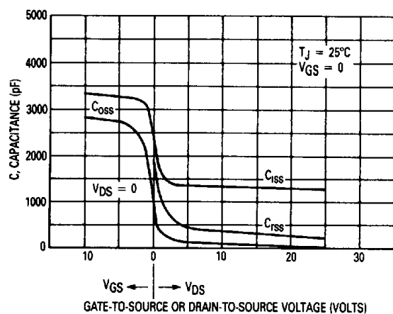
Figure 11. Capacitance Variation
