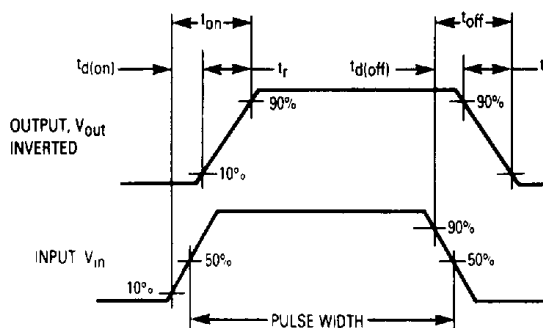
Figure 14. Switching Waveforms
