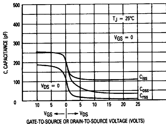
Figure 11. Capacitance Variation
