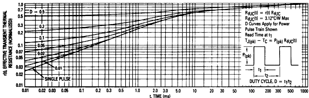
Figure 9. Thermal Response
