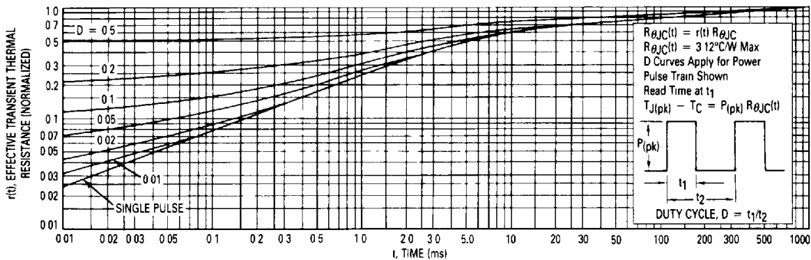
Figure 9. Thermal Response
