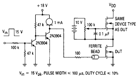
Figure 17. Gate Charge Test Circuit
